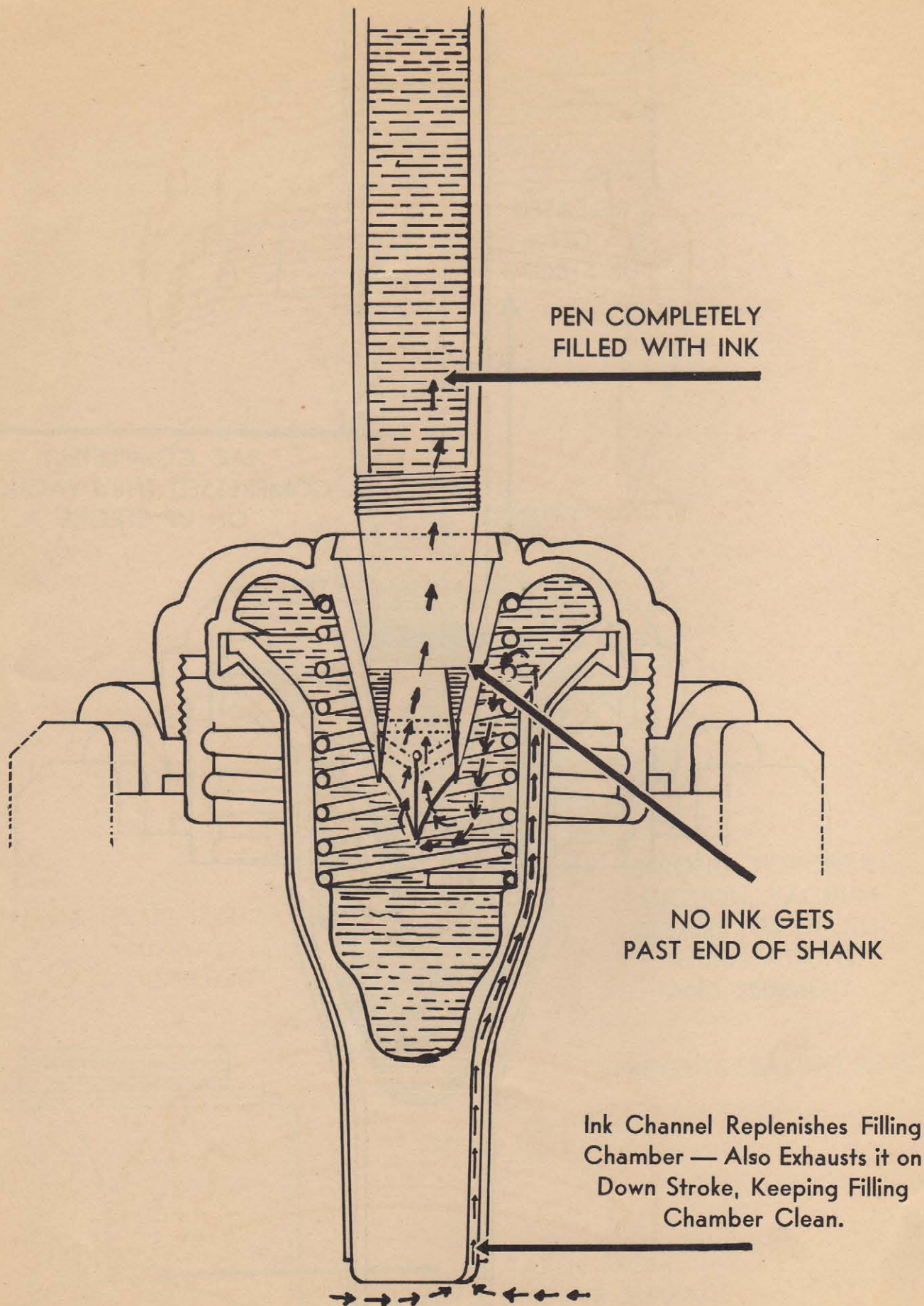
FOURTH — Atmospheric pressure forces ink into pen, filling more completely than pen's own mechanism.
